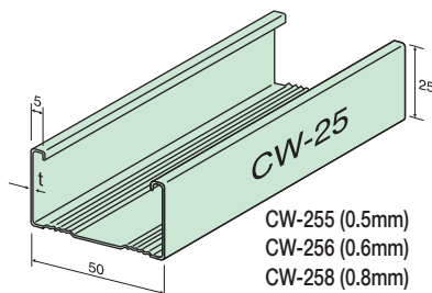
Double Furring
