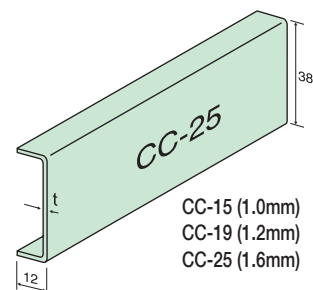
Carrying Channel
